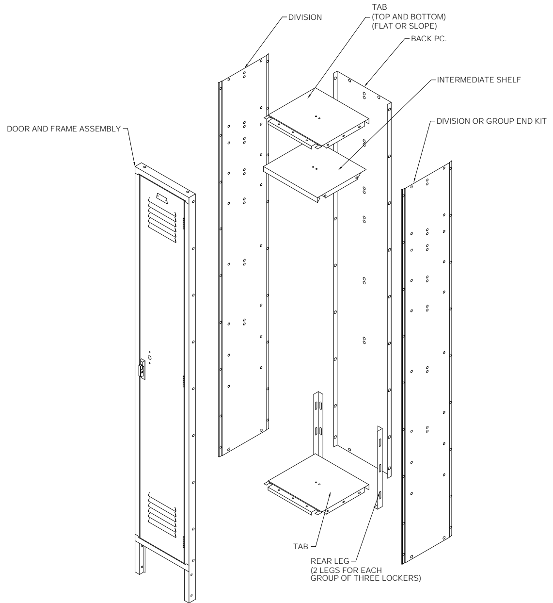
COMMON SINGLE TIER LOCKER EXPLODED VIEW
