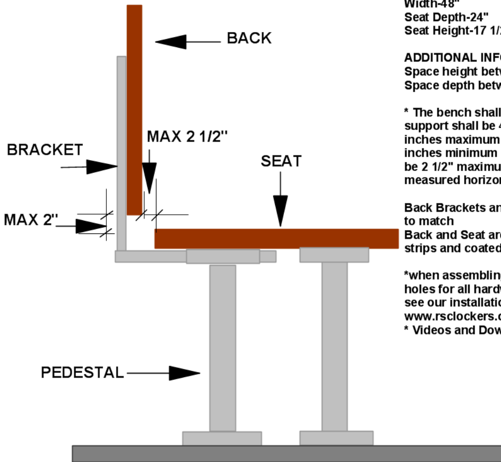
SIDE ELEVATION
